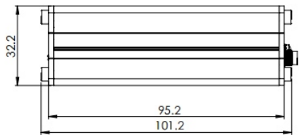
Right view
